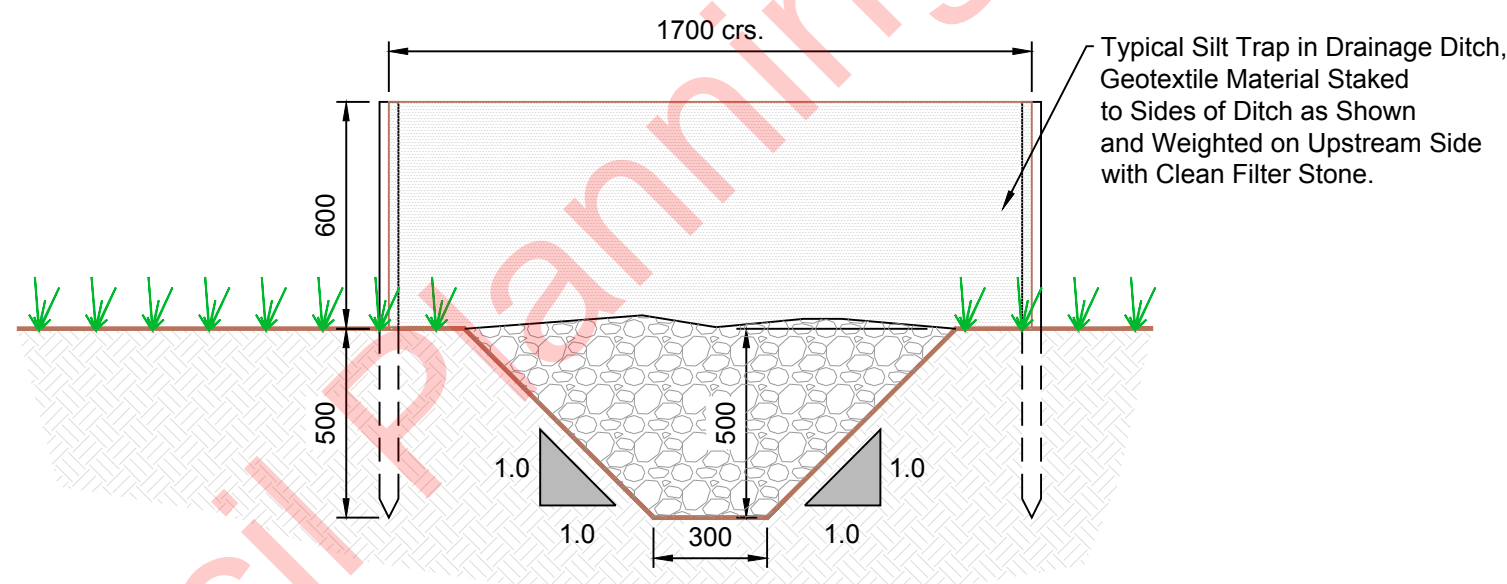
SILT TRAP IN DRAINAGE DITCH
